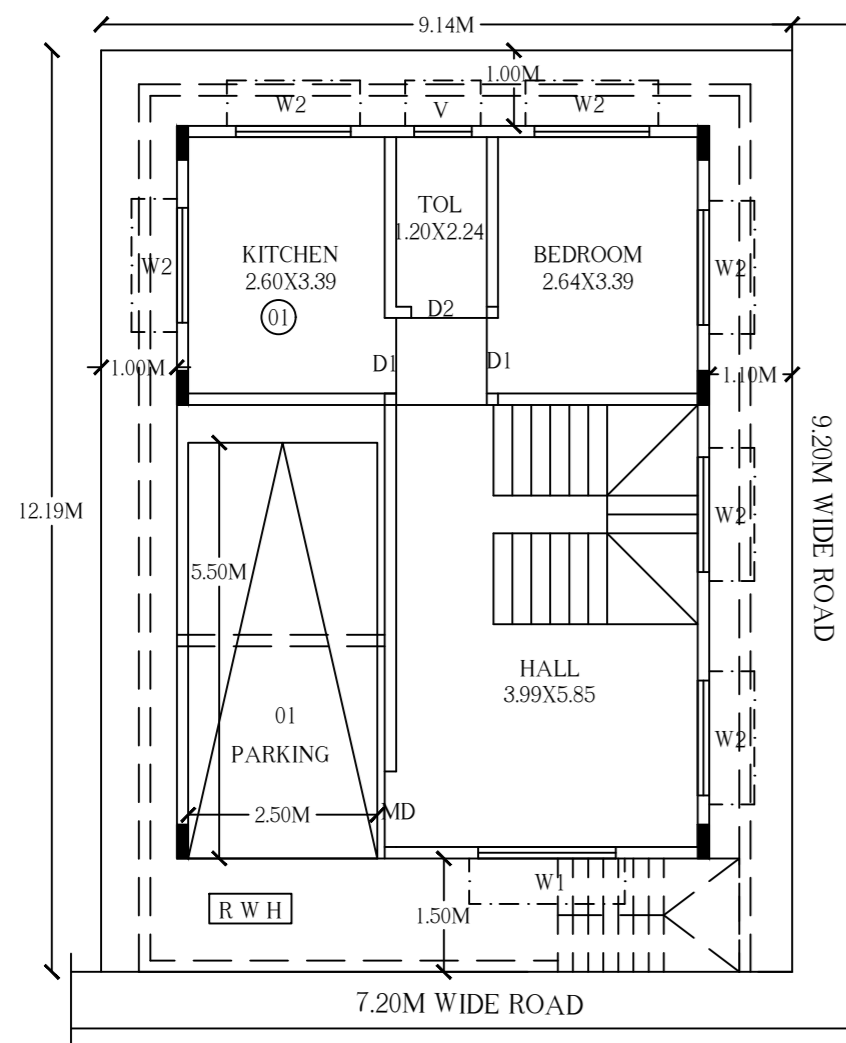
ALTERATIONS TO EXISTING GROUND FLOOR PLAN
