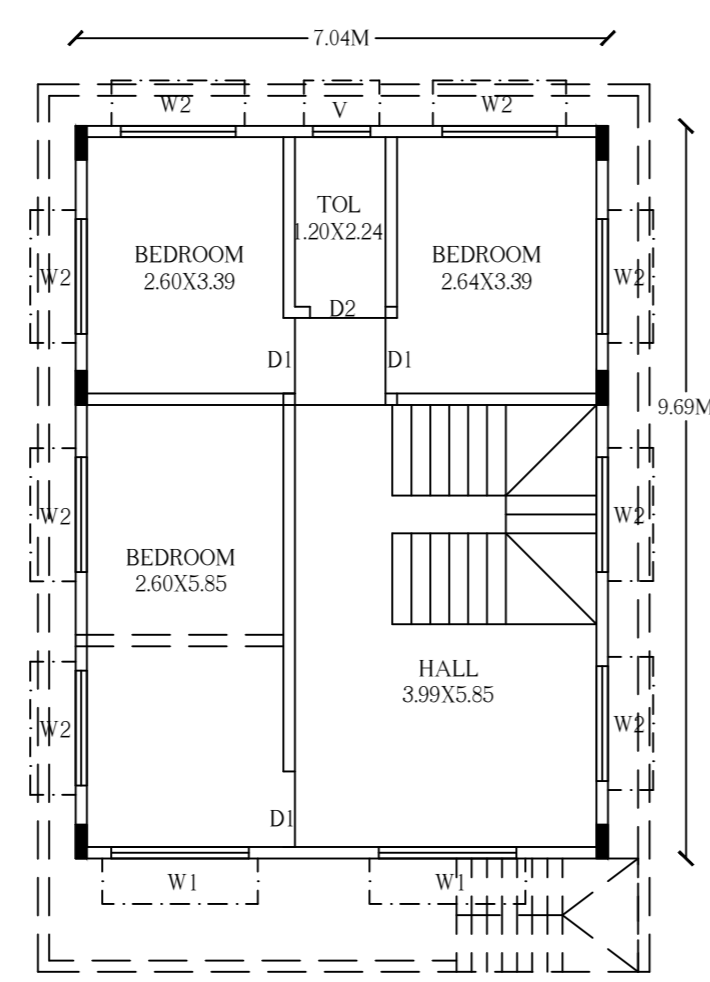
ALTERATIONS TO EXISTING FIRST FLOOR PLAN
